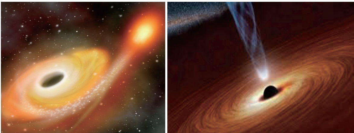
Left: Imaginary scene of a tidal disruption event – A black hole is depicted preying on a star.
