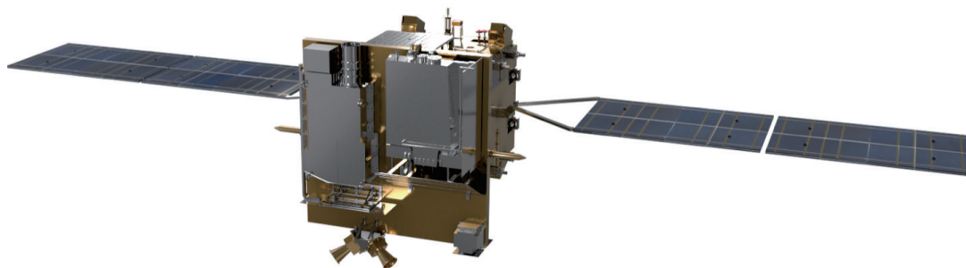
Illustration of ASO-S, the first Chinese solar mission to be launched in 2022. (Image by ASO-S Team)
