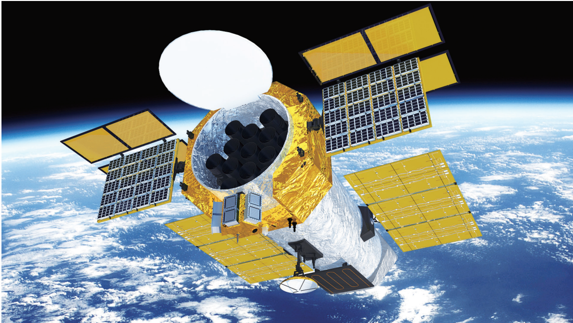
Illustration of eXTP, flagship space astronomy mission developed by a Sino-European scientific consortium led by the Institute of High Energy Physics (IHEP), CAS. For more information, please refer to page 10 of Issue 1, 2018 of BCAS . (Image by courtesy of IHEP, CAS)
